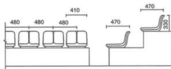
SJ-A005 中靠背中空塑料椅 SJ-A005 Middle-Backrest Hollow Plastic Chair
