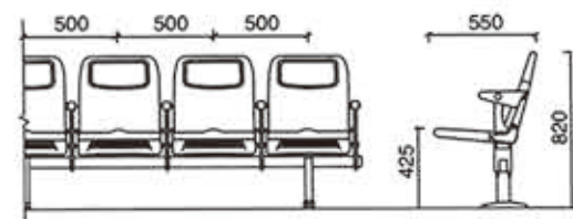
SJ-A018 落地式带扶手中空塑料翻板椅 SJ-A018 Floor-Standing Hollow Plastic Folding Chair With Armrests
