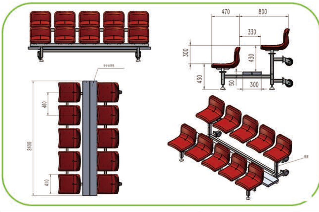
SJ-A070 Movable Assembled Stand
