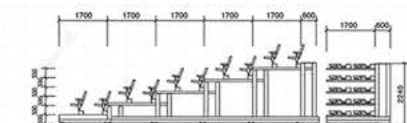
SJ-A033 Rear-Mounted Single-Layer Double-Row Grandstand Layer width: 1700mm Layer Height: 330mm Seat Type: Postposition type plastic plate turning chair Seat pitch: 500mm Drive mode: manual or electric Seats flip modes: Manual or auto flip
