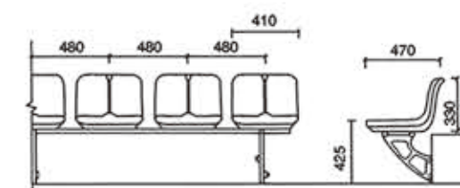
SJ-A009 悬挂式中靠背中空塑料椅 SJ-A009 Hanging Middle-Backrest Hollow Plastic Chair
