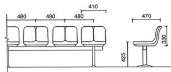
SJ-A006 落地式中靠背中空塑料椅 SJ-A006 Floor-Standing Middle-Backrest Hollow Plastic Chair
