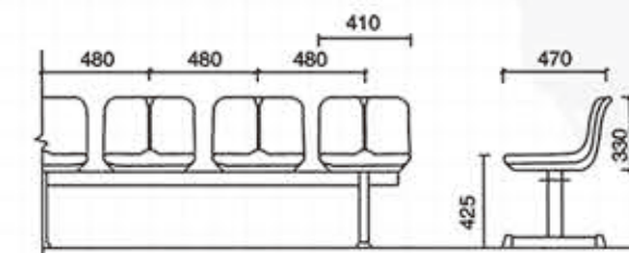
SJ-A007 移动式中靠背中空塑料椅 SJ-A007 Mobile Middle-Backrest Hollow Plastic Chair ( Square Column Bracket )
