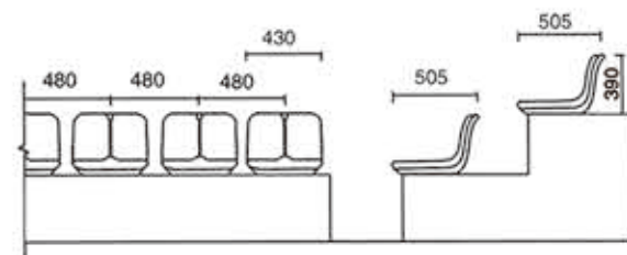
SJ-A011 高靠背中空塑料椅 SJ-A011 High Backrest Hollow Plastic Chair
