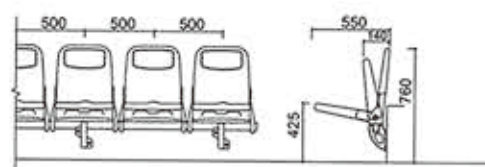
SJ-A017 悬挂式无扶手中空塑料翻板椅 SJ-A017 Hanging Armless Hollow Plastic Folding Chair
