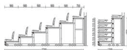
SJ-A031 前置软包翻版椅 SJ-A031 Front upholstery copy chair Width:900mm Height:310mm Seat Type: Flip-over chair with front soft bag Seat Pitch:500mm Drive Mode: Manual or Electric Seat Flip Test: Manual or Automatic
