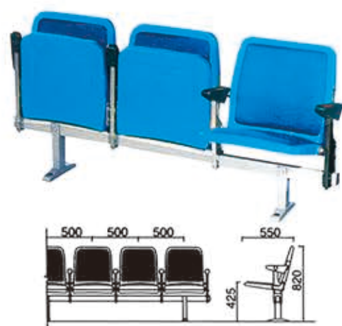
SJ-A019 落地式带扶手中空软包塑料翻板椅 SJ-A019 Floor-Standing Hollow Soft Plastic Folding Chair With Armrests
