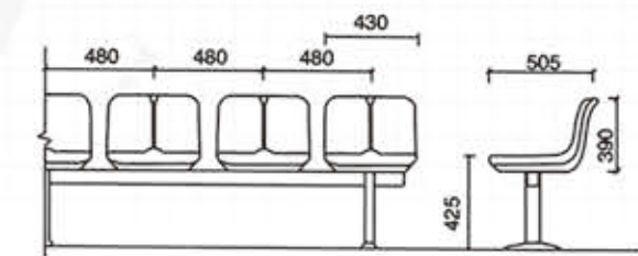
SJ-A014 落地式高靠背中空塑料椅 SJ-A014 Floor-Standing High Backrest Hollow Plastic Chair
