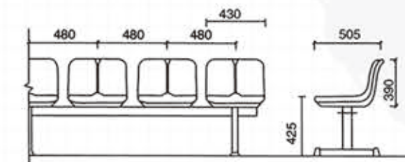
SJ-A013 移动式高靠背中空塑料椅 SJ-A013 Mobile High Backrest Hollow Plastic Chair
