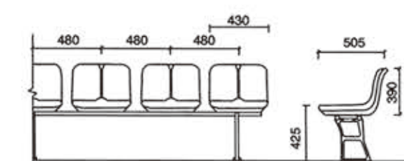
SJ-A016 直立式高靠背中空塑料椅 SJ-A016 Upright High Backrest Hollow Plastic Chair
