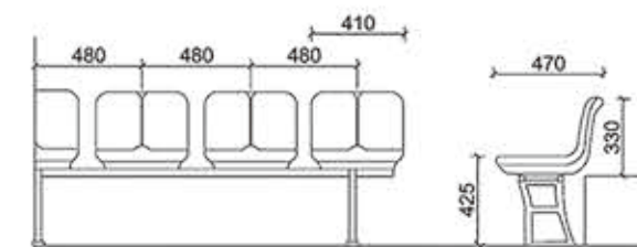
SJ-A010 直立式中靠背中空塑料椅 SJ-A010 Upright Middle-Backrest Hollow Plastic Chair
