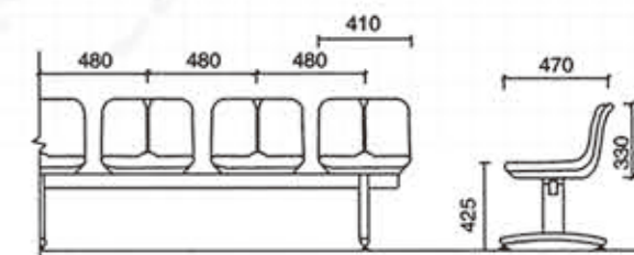
SJ-A008 移动式中靠背中空塑料椅 SJ-A008 Mobile Middle-Backrest Hollow Plastic Chair ( Oval Column Bracket )
