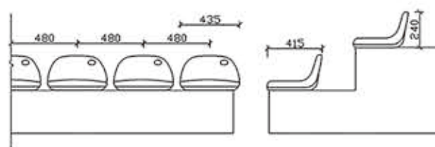
SJ-A012 中空塑料椅 SJ-A012 Hollow Plastic Chair
