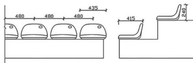
SJ-A012 中空塑料椅 SJ-A012 Hollow Plastic Chair
