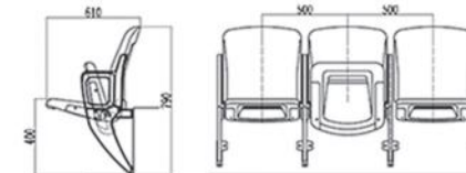
SJ-A022 侧装式翻板椅 SJ-A022 Side Mounted Folding Chair
