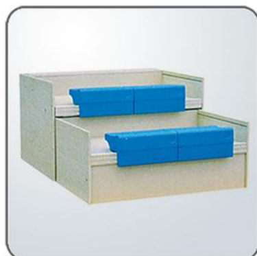
SJ-A030 中空长条凳伸缩看台 Hollow Bench Telescopic Bleachers Width:700mm Height:280mm Seat Type:Long Hollow Stool Without Backrest Seat Pitch:460mm Drive Mode: Manual or Electric
