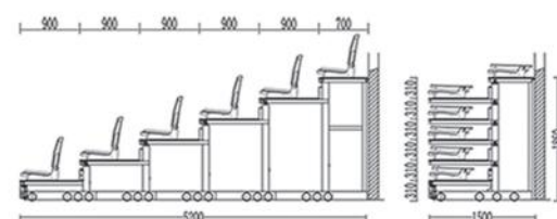
SJ-A031 前置软包翻版椅 SJ-A031 Front upholstery copy chair Width:900mm Height:310mm Seat Type: Flip-over chair with front soft bag Seat Pitch:500mm Drive Mode: Manual or Electric Seat Flip Test: Manual or Automatic
