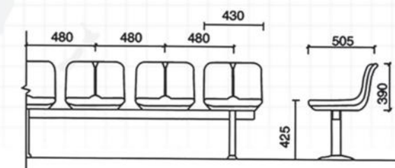
SJ-A014 落地式高靠背中空塑料椅 SJ-A014 Floor-Standing High Backrest Hollow Plastic Chair
