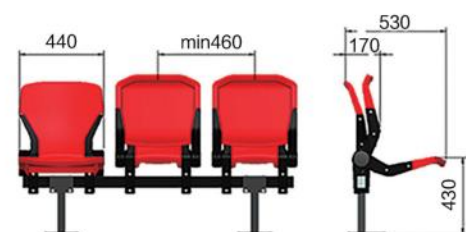
SJ-A050 Upright Stadium Seat
