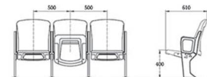
SJ-A021 直立式翻板椅 SJ-A021 Upright Folding Chair
