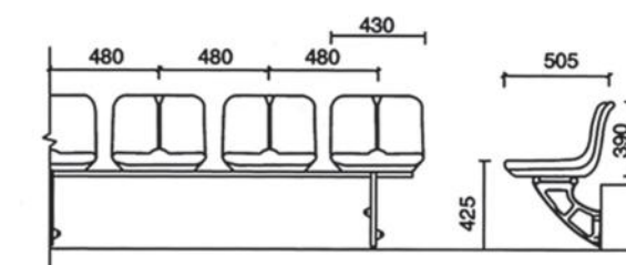
SJ-A015 悬挂式高靠背中空塑料椅 SJ-A015 Hanging High Backrest Hollow Plastic Chair
