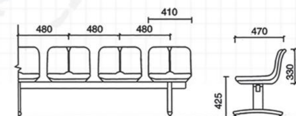
SJ-A008 移动式中靠背中空塑料椅 SJ-A008 Mobile Middle-Backrest Hollow Plastic Chair ( Oval Column Bracket )
