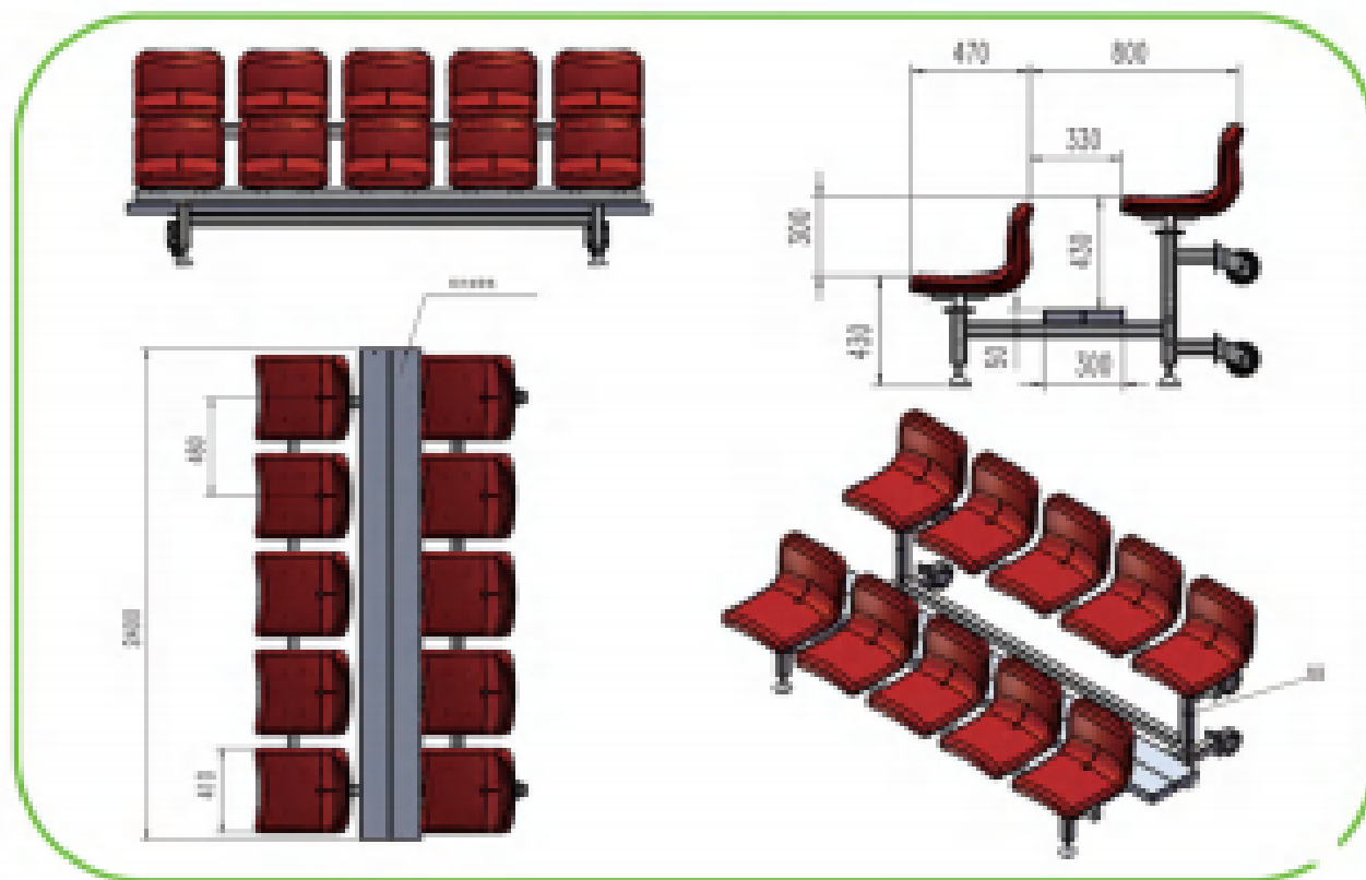
SJ-A070 Movable Assembled Stand
