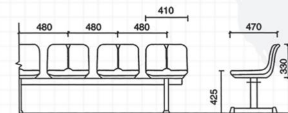
SJ-A007 移动式中靠背中空塑料椅 SJ-A007 Mobile Middle-Backrest Hollow Plastic Chair ( Square Column Bracket )
