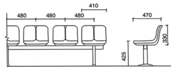
SJ-A006 落地式中靠背中空塑料椅 SJ-A006 Floor-Standing Middle-Backrest Hollow Plastic Chair
