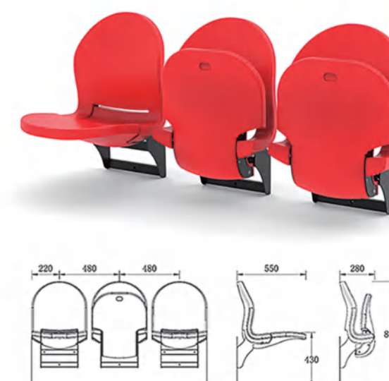
SJ-A040 海洋座椅 SJ-A040 Ocean Folding Chair
